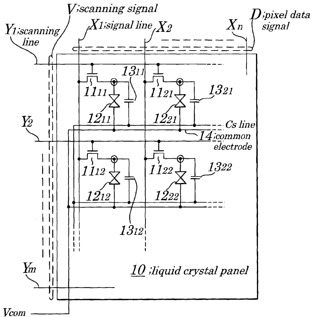
FIG. 12 (PRIOR ART)
