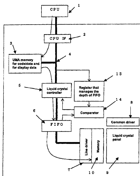
Liquid crystal display apparatus
