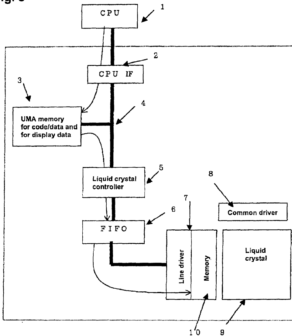
Liquid crystal display apparatus
