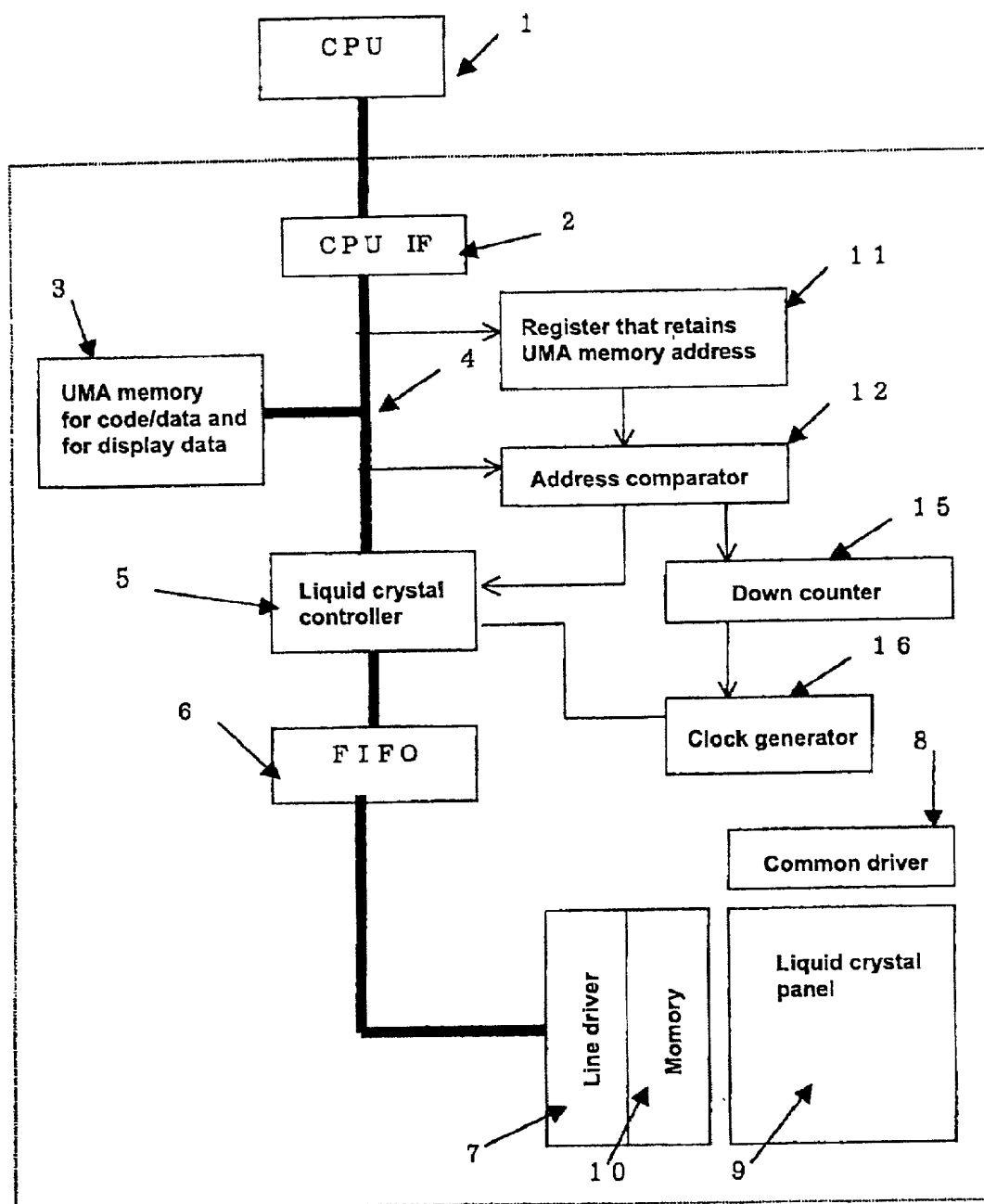
Liquid crystal display apparatus
