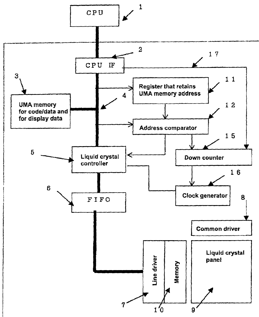
Liquid crystal display apparatus
