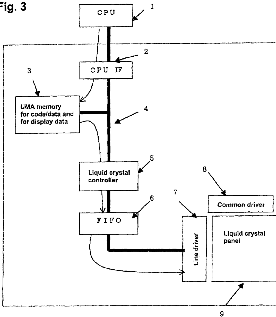
Liquid crystal display apparatus
