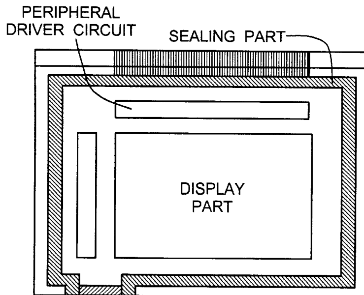
STRUCTURE OF CONVENTIONAL PANEL
