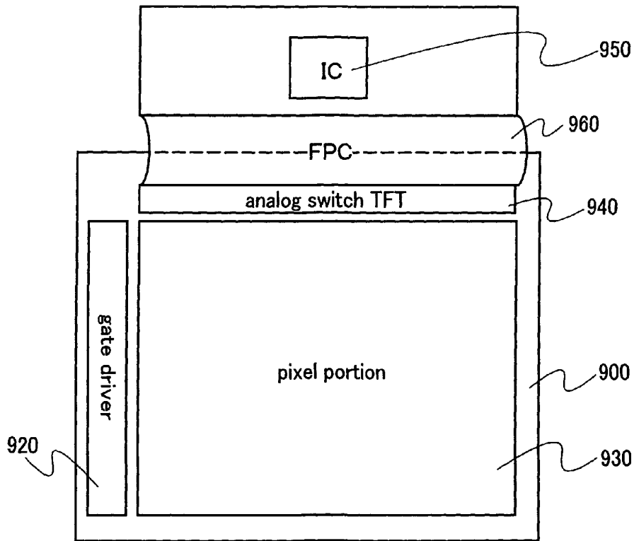
FIG. 17A IC connected by FPC
