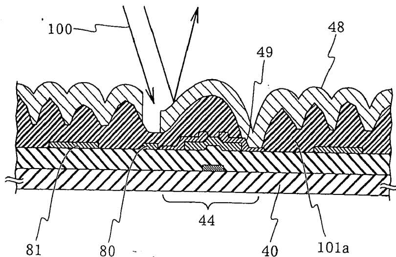
FIG. 13(a) REFLECTIVE LIQUID CRYSTAL DISPLAY APPARATUS
