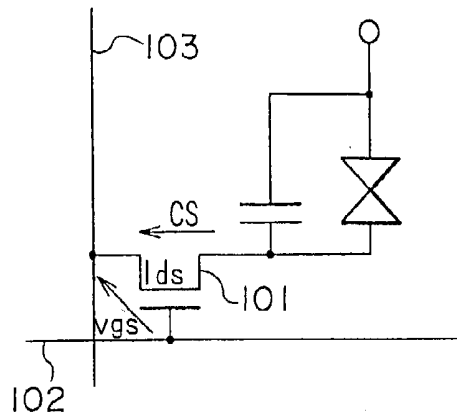
FIG. 25 RELATED ART
