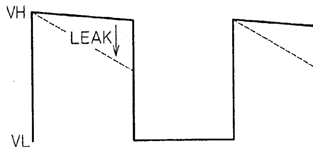
FIG. 25 RELATED ART
