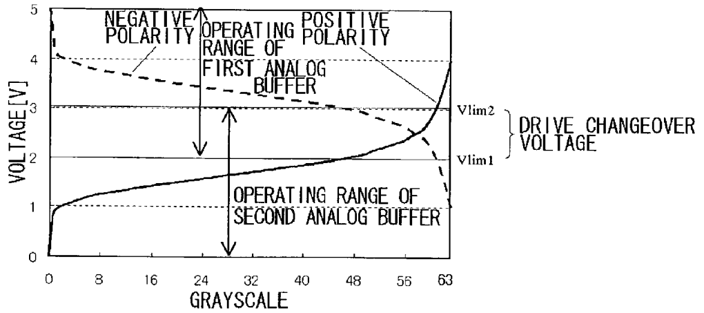
CIRCUIT OPERATING RANGE (GAMMA-MODULATED STATE) IN COMMON INVERSION DRIVE
