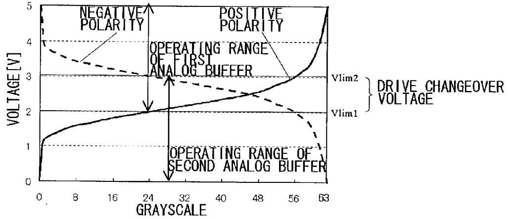
LIQUID CRYSTAL GAMMA CHARACTERISTIC AND DRIVER-CIRCUIT OPERATING RANGE (STANDARD STATE) INCOMMON INVERSION DRIVE
