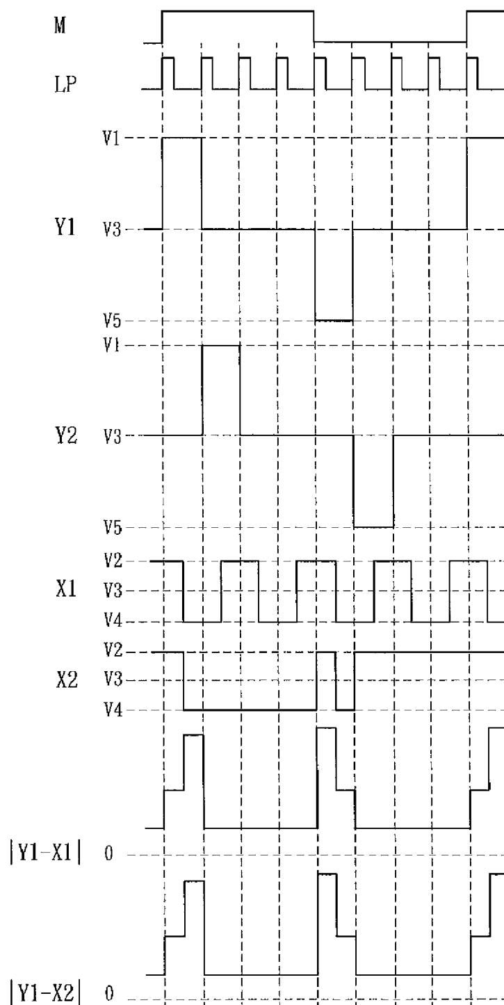
Fig . 3 PRIOR ART
