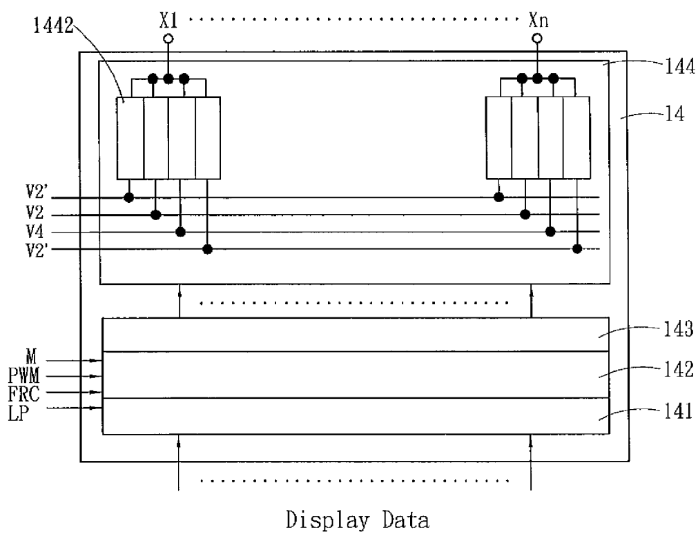
Fig . 8 PRIOR ART
