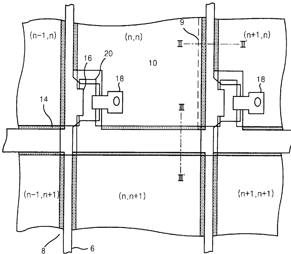
FIG. 1 CONVENTIONAL ART
