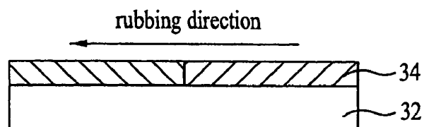
FIG. 13C Related Art
