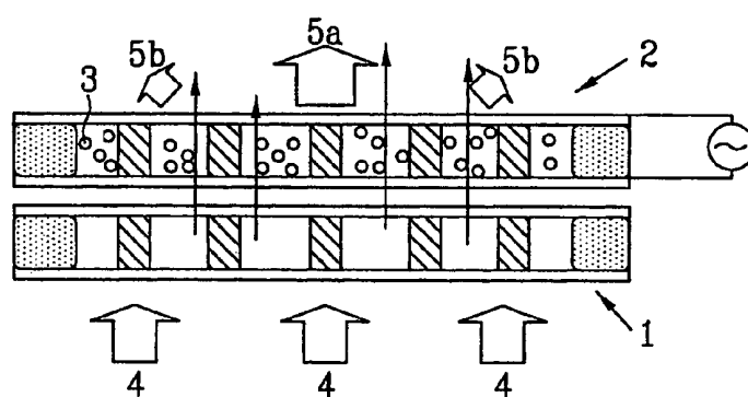
FIG. 1C Related Art
