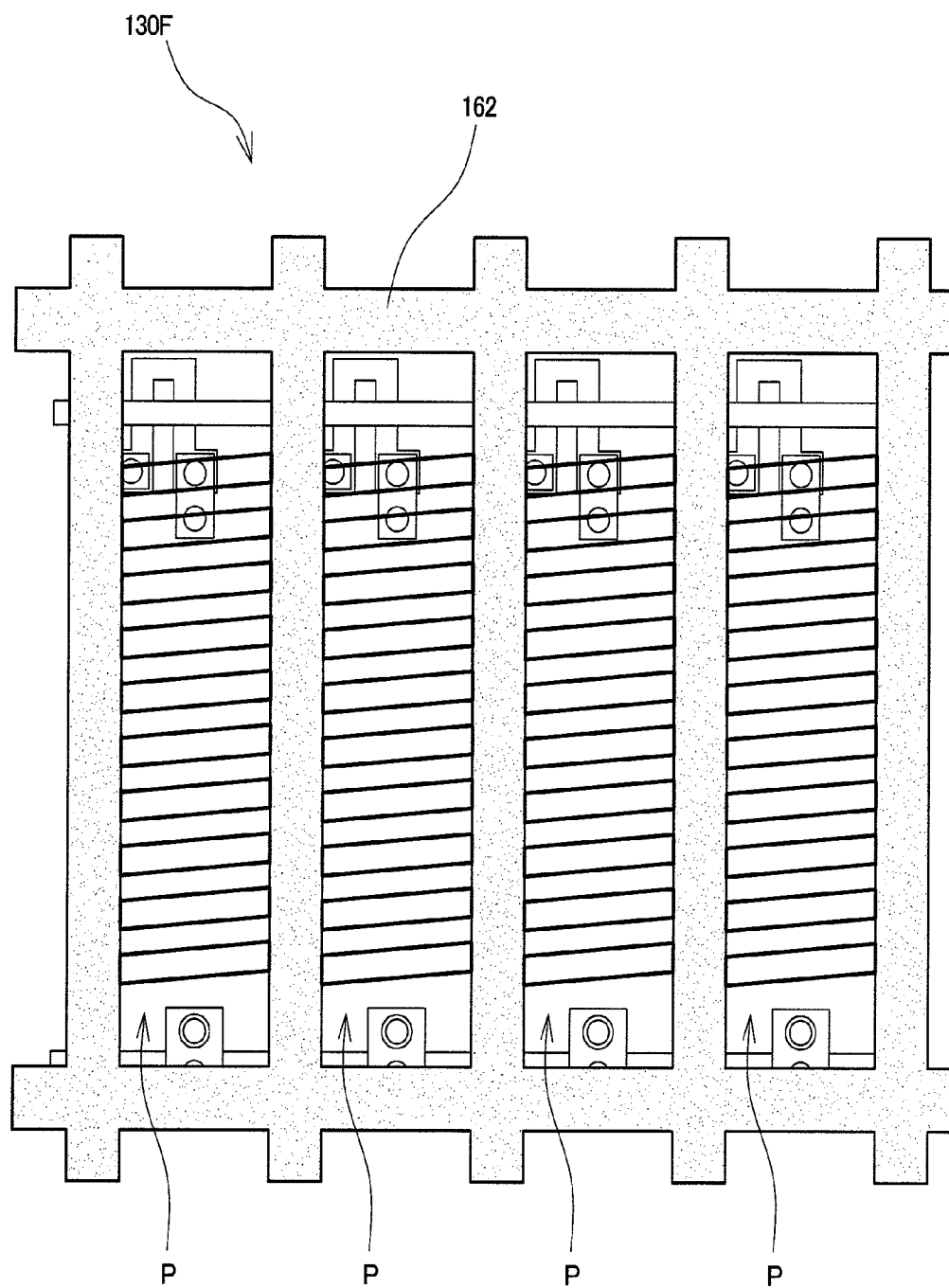
FIG. 17 (PRIOR ART)
