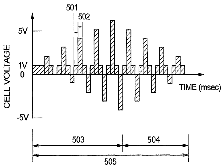
DRIVING WAVEFORM
