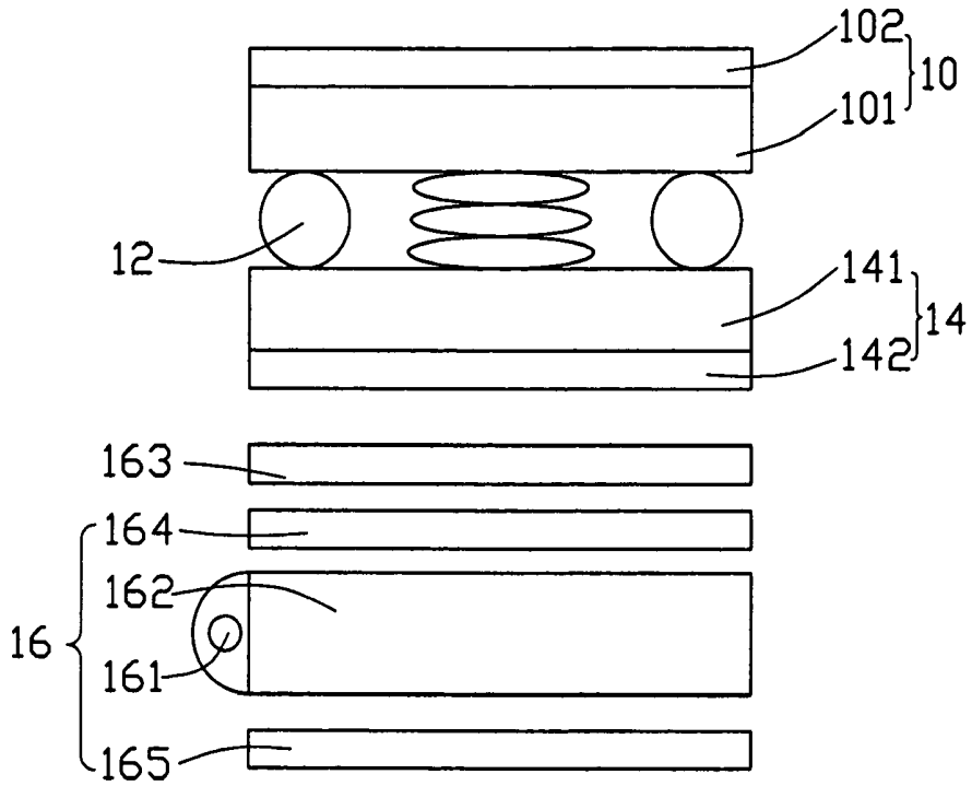
FIG. 5 (PRIOR ART)
