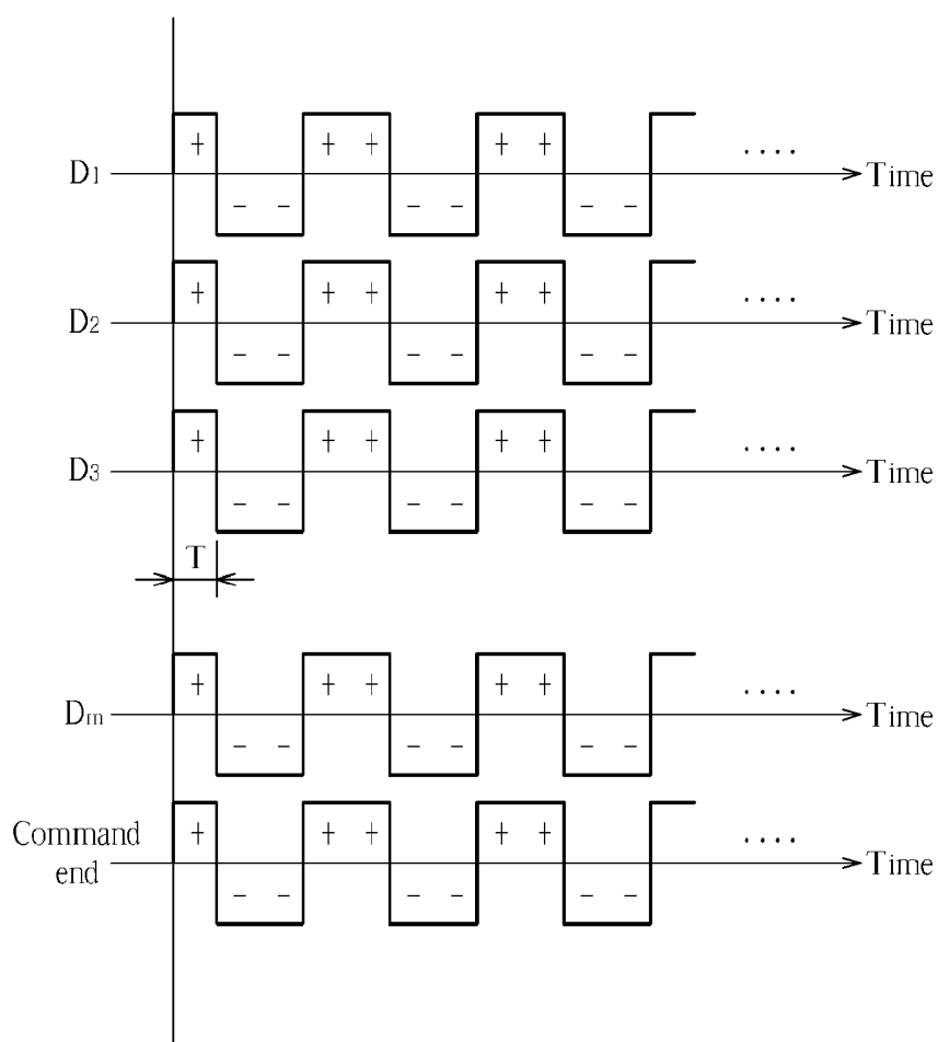
FIG. 4 PRIOR ART
