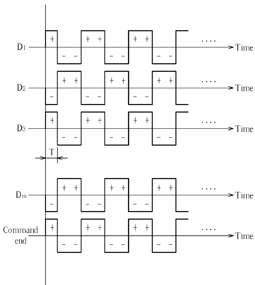
FIG. 6 PRIOR ART
