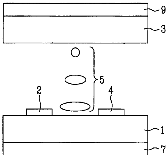
FIG. 3C Related Art
