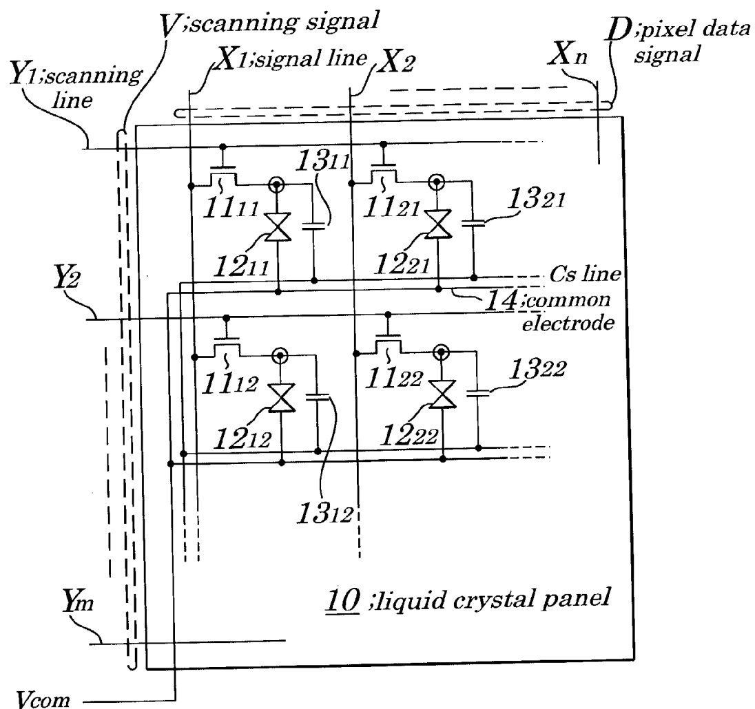
FIG. 12 (PRIOR ART)
