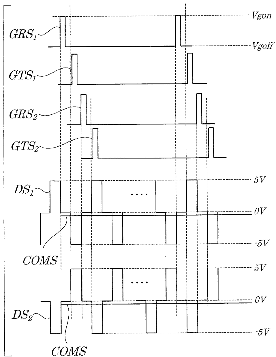
FIG. 17(RELATED ART)
