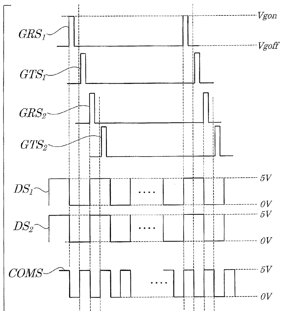
FIG. 18(RELATED ART)
