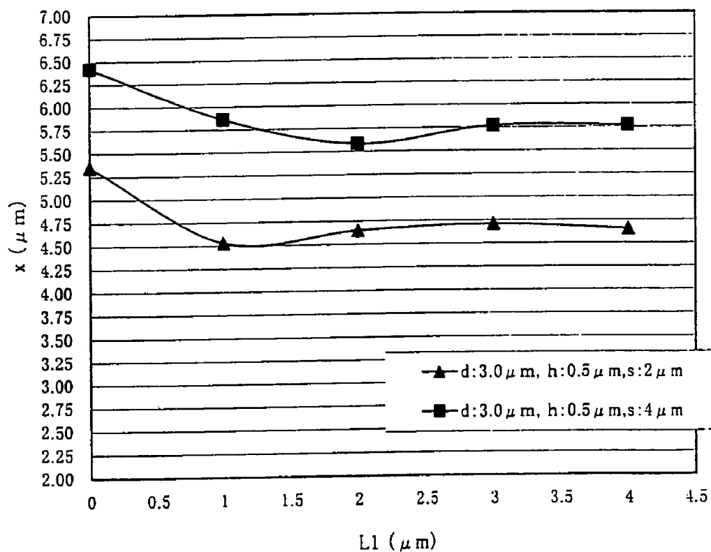
FIG. 11B (cell gap 3.0 \mu\text{m} )
