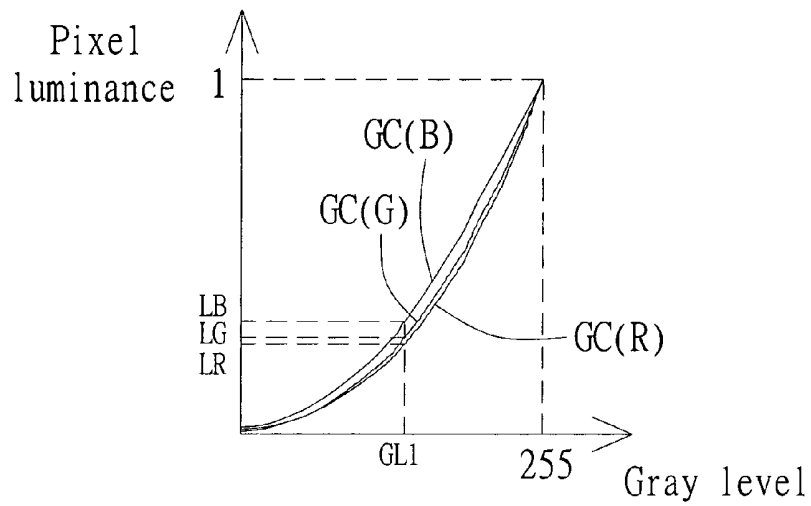
FIG. 2(PRIOR ART)
