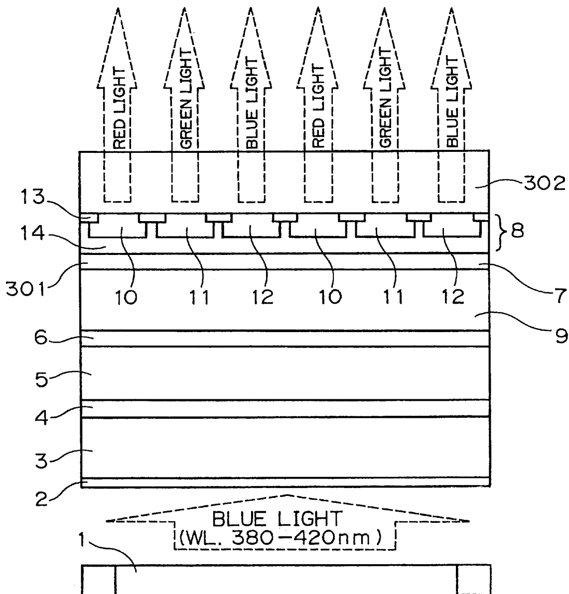
FIG. 3 PRIOR ART
