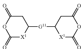
Chemical formula 16:
