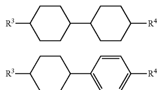
Chemical formula 6:
