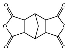
Chemical formula 68:
