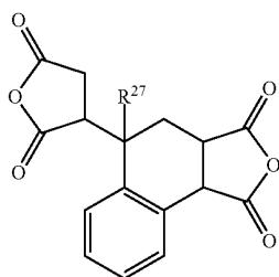
Chemical formula 65:
