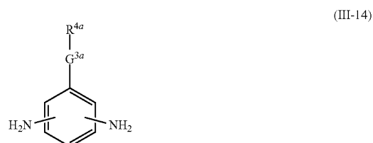
Chemical formula 14:
