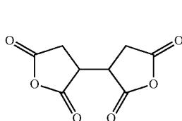
Chemical formula 28:
