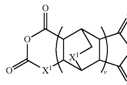
Chemical formula 21:
