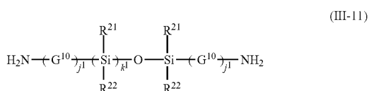
Chemical formula 12:
