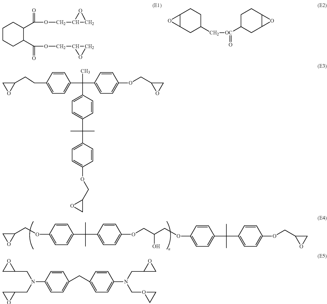
Chemical formula 95:
