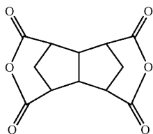
Chemical formula 25:
