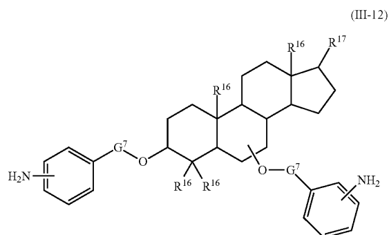
Chemical formula 13:
