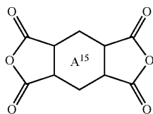
Chemical formula 61:
