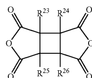
Chemical formula 17:
