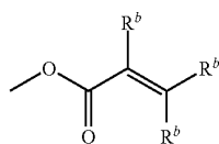
Chemical formula 29:
