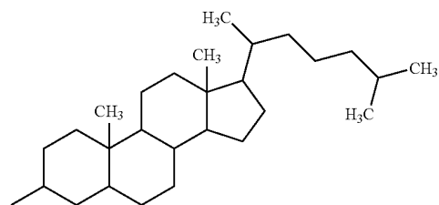
Chemical formula 15:
