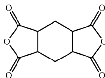
Chemical formula 62:
