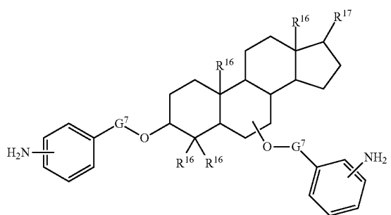
Chemical formula 13:
