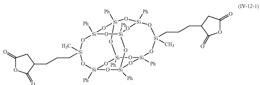
Chemical formula 79:
