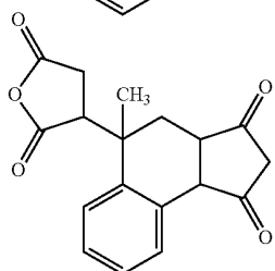
Chemical formula 67:
