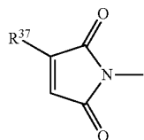
Chemical formula 92:
