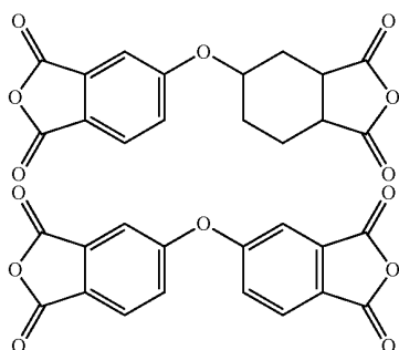
Chemical formula 65:
