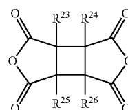
Chemical formula 59:
