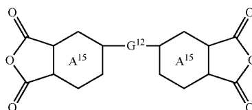
Chemical formula 63:
