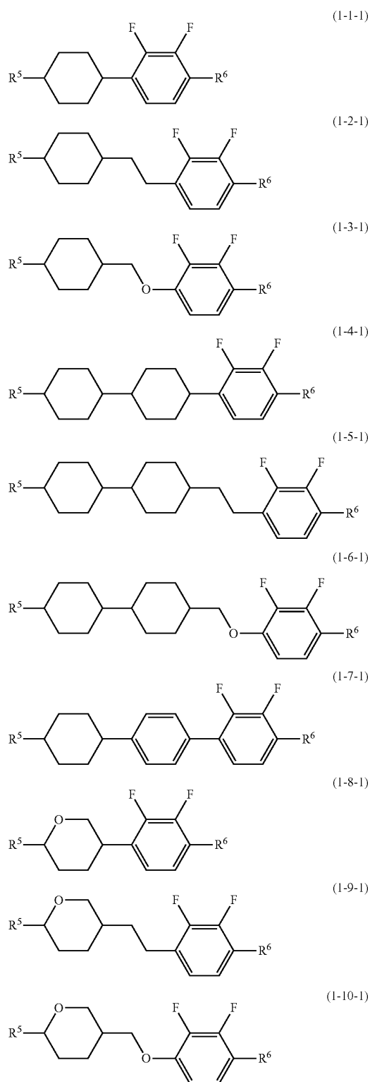
Chemical formula 30:
