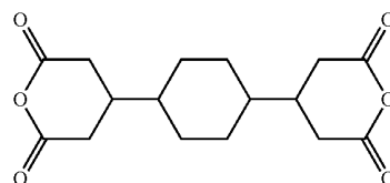
Chemical formula 59:
