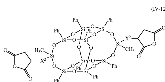
Chemical formula 27:
