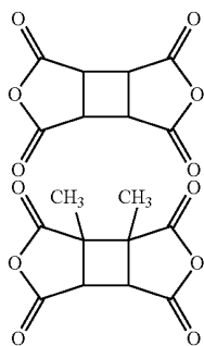
Chemical formula 60:
