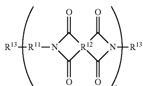
Chemical formula 7:
