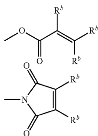
Chemical formula 81:
