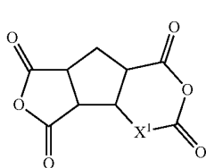
Chemical formula 22:
