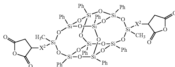
Chemical formula 27:
