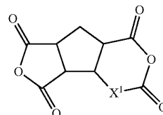
Chemical formula 22:
