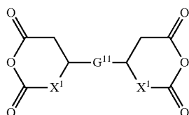
Chemical formula 16:
