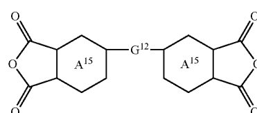
Chemical formula 19:
