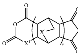
Chemical formula 67:
