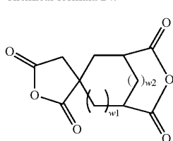
Chemical formula 24:
