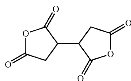
Chemical formula 58:
