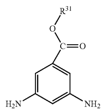
Chemical formula 47:
