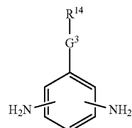
Chemical formula 9:
