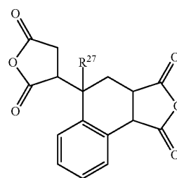
Chemical formula 20:
