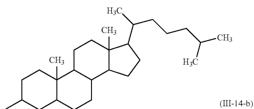
Chemical formula 15:
