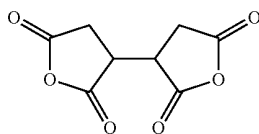
Chemical formula 28:
