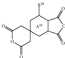
Chemical formula 23:
