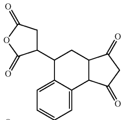
Chemical formula 66:
