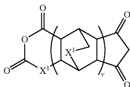
Chemical formula 21:
