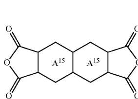
Chemical formula 26:
