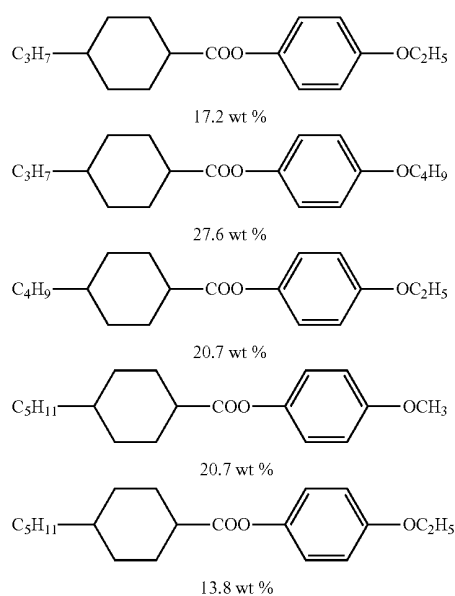
Chemical formula 96:
