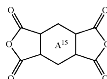
Chemical formula 18:
