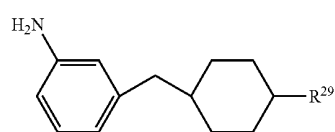
Chemical formula 46:
