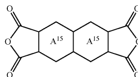
Chemical formula 26:
