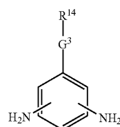
Chemical formula 42:
