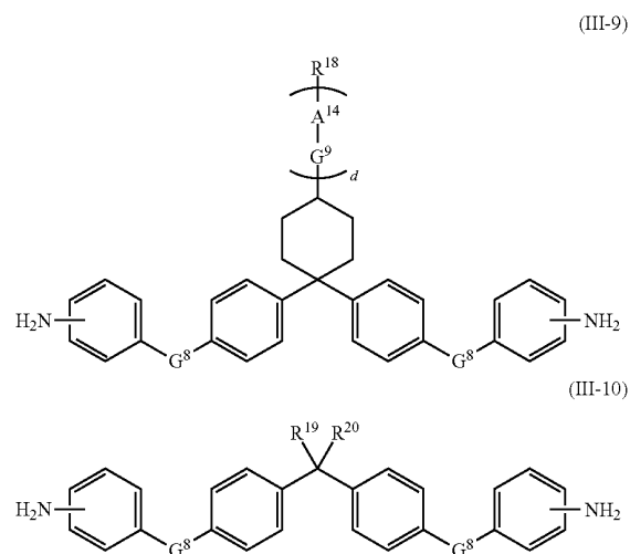
Chemical formula 44:
