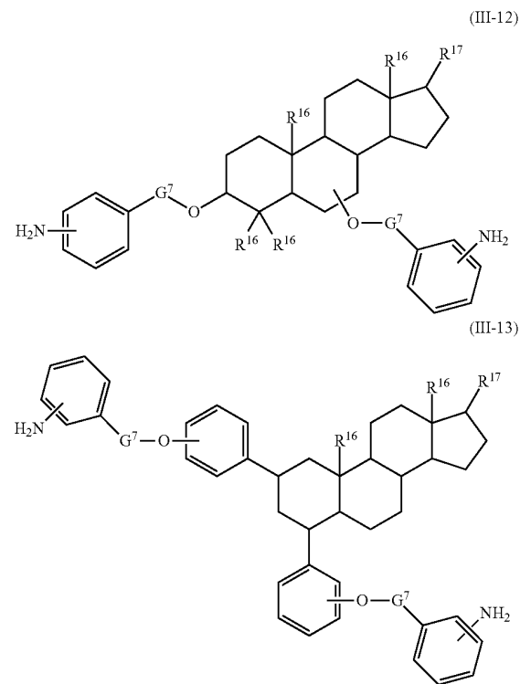
Chemical formula 45:
