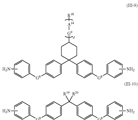
Chemical formula 11:
