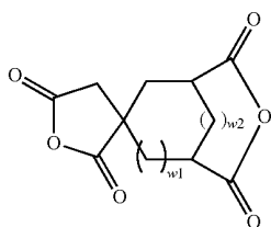
Chemical formula 24:
