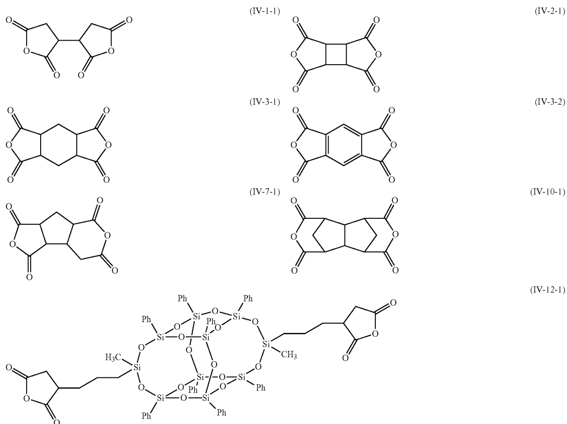
Chemical formula 80:
