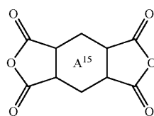
Chemical formula 18:
