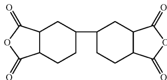
Chemical formula 64:
