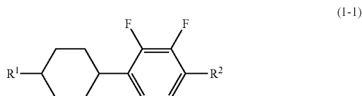
Chemical formula 2:
