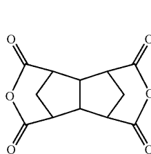
Chemical formula 26:
