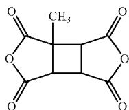
Chemical formula 61:
