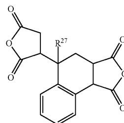
Chemical formula 20:
