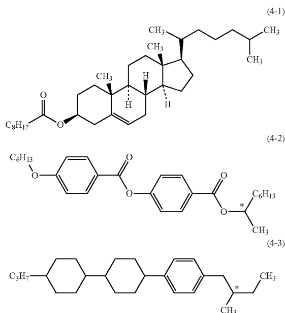
Chemical formula 93:
