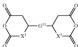
Chemical formula 57:
