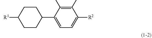
Chemical formula 2:
