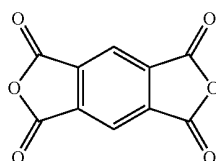
Chemical formula 63:
