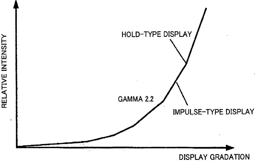
GAMMA CHARACTERISTICS OF LIQUID CRYSTAL DISPLAY
