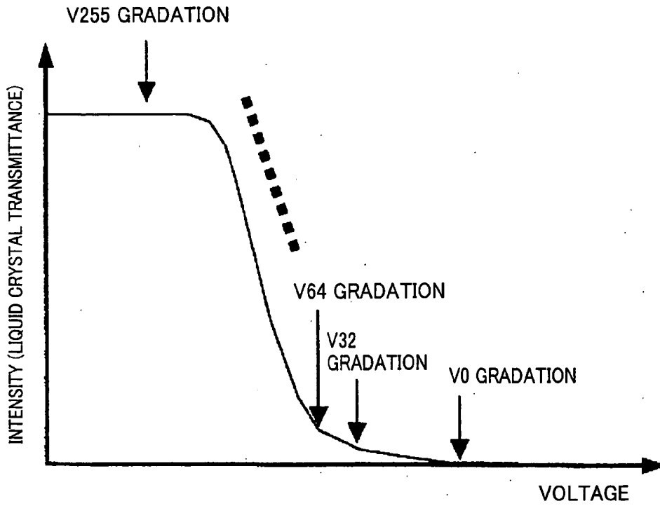
V-T CHARACTERISTICS OF LIQUID CRYSTAL DISPLAY PANEL AND VOLTAGES
