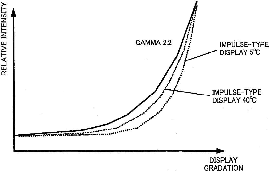
GAMMA CHARACTERISTICS OF LIQUID CRYSTAL DISPLAY
