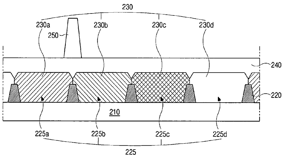
FIG. 3 RELATED ART
