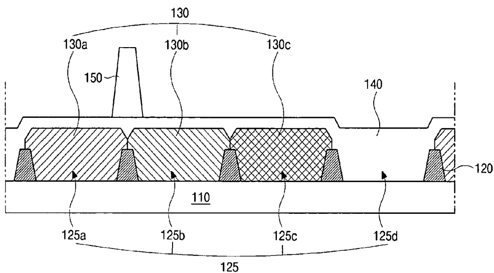
FIG. 2 RELATED ART
