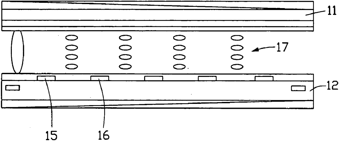
FIG. 5 (PRIOR ART)
