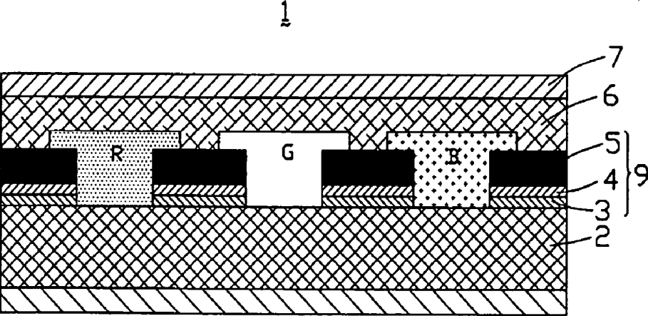
FIG. 5 (PRIOR ART)
