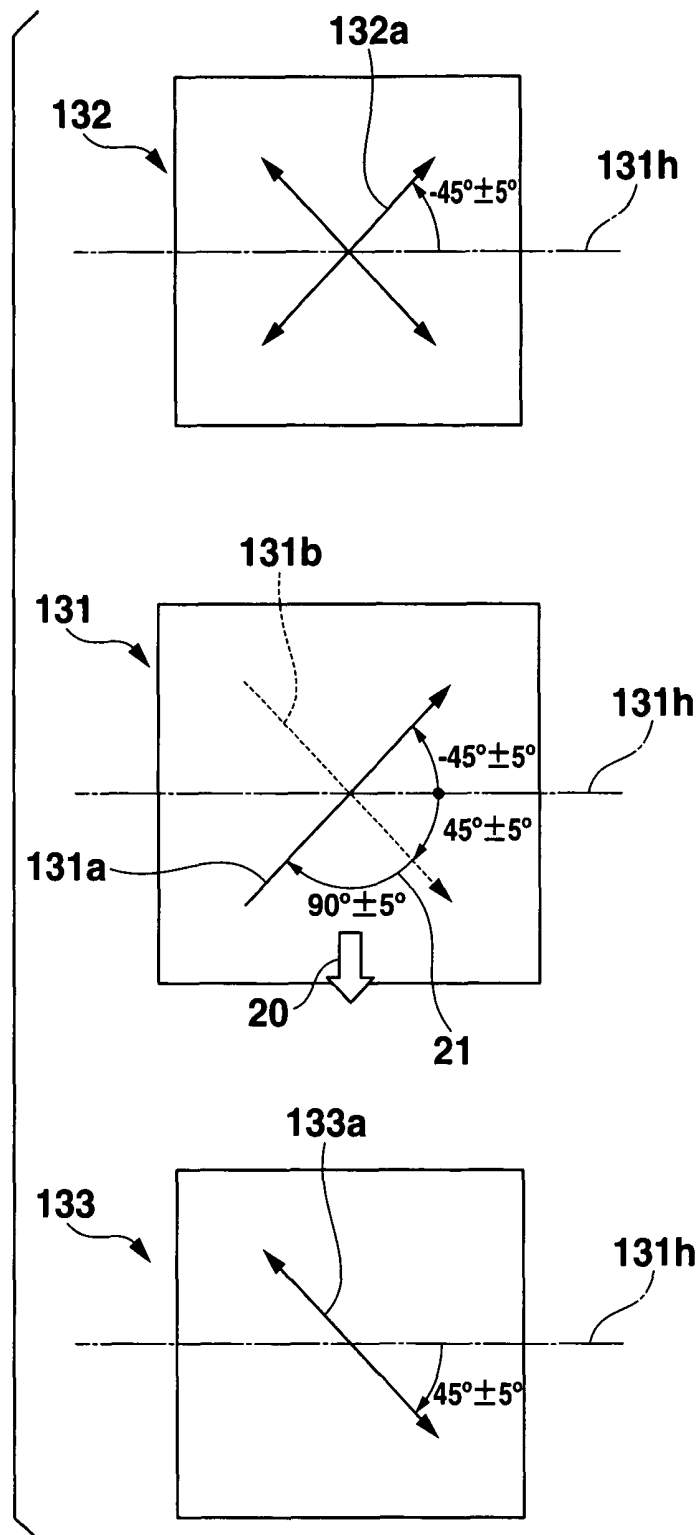
FIG.13 RELATED ART
