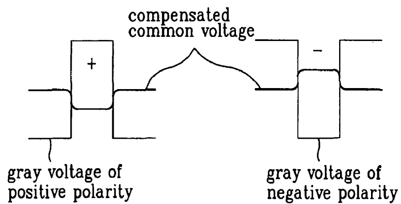
FIG. 5 Related Art
