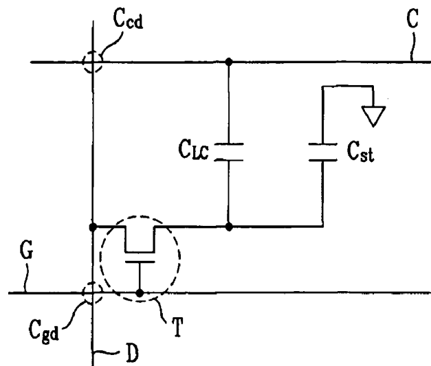
FIG. 2 Related Art
