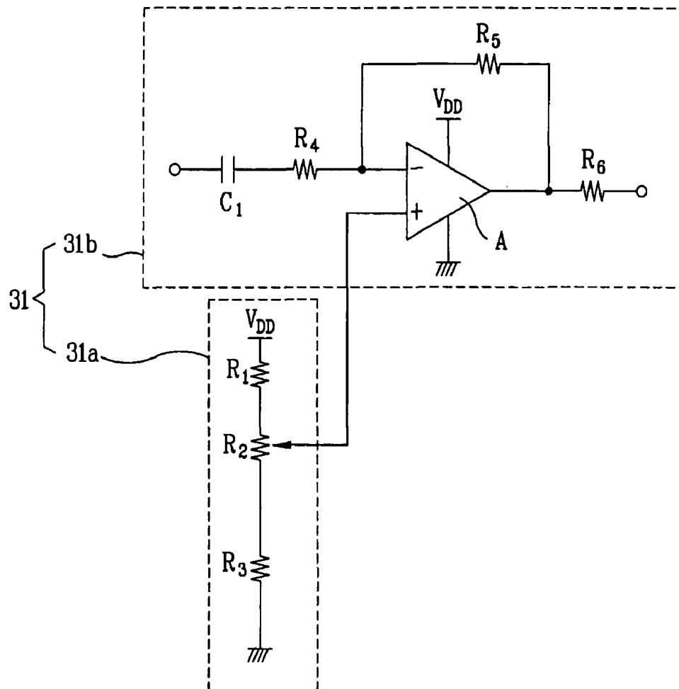
FIG. 5 Related Art
