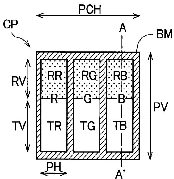
FIG. 11 PRIOR ART
