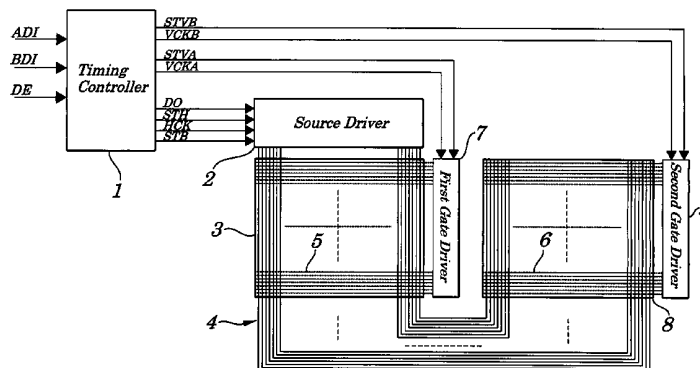
100 :Liquid Crystal Display Device
