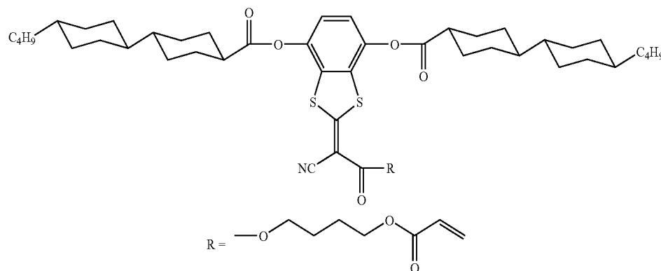
Rod-like liquid crystal compound (2)
