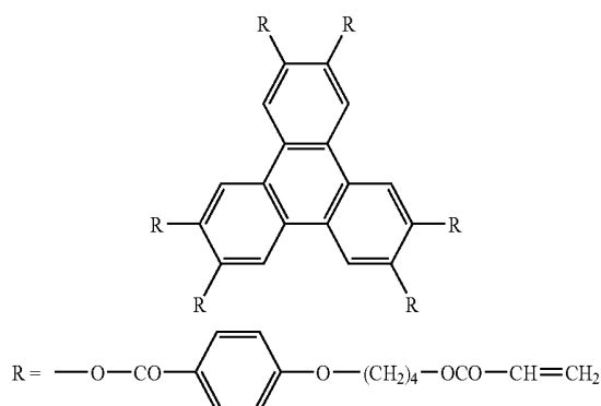
Discotic liquid crystalline compound
