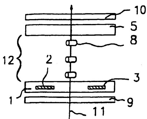
FIG. 1c PRIOR ART
