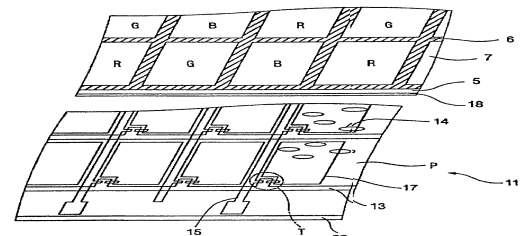
(related art) FIG 1A
