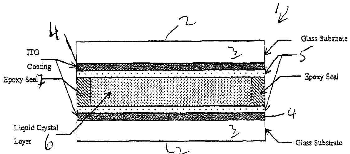
Fig. 1 Structure of passively driven liquid crystal display
