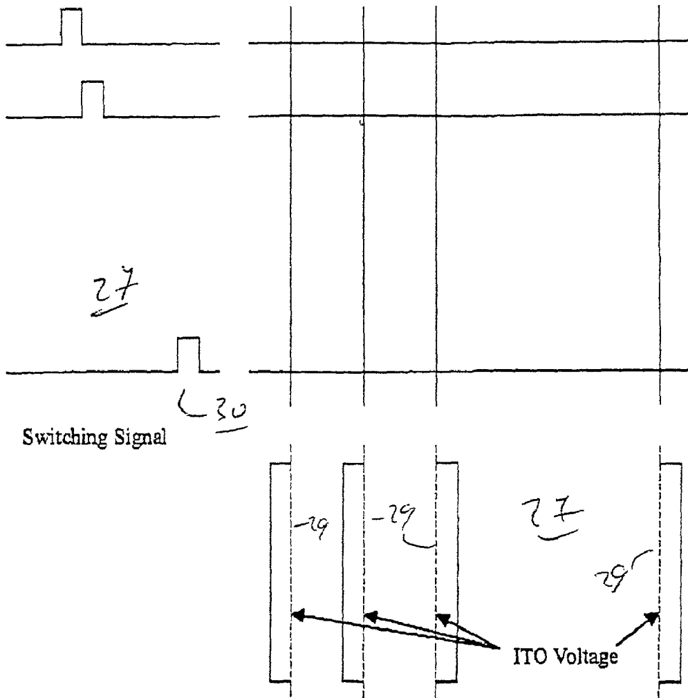
Fig. 20 Signal waveform incorporating 2-column inversion scheme for actively driven liquid crystal display
