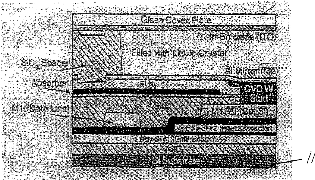
Fig. 6 Arrangement for reflective single crystal CMOS microdisplay
