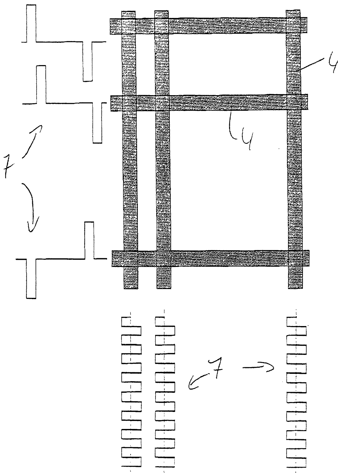
Fig. 2 Example waveform applied to the common and segment electrodes
