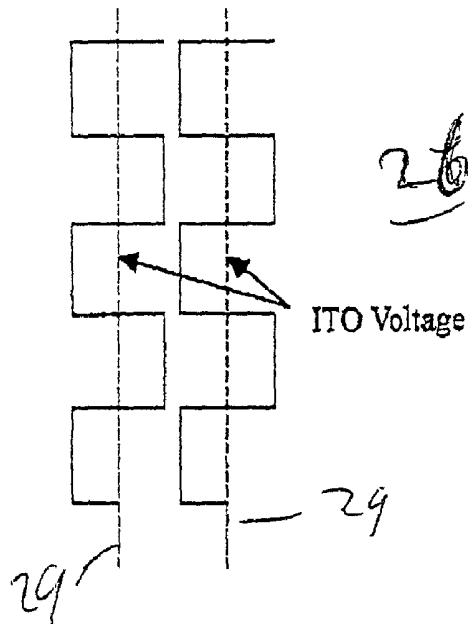
Fig. 19 Signal waveform incorporating 2-row inversion scheme for actively driven liquid crystal display
