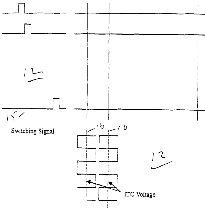
Fig. 7 Signal waveform incorporating row inversion scheme for actively driven liquid crystal display
