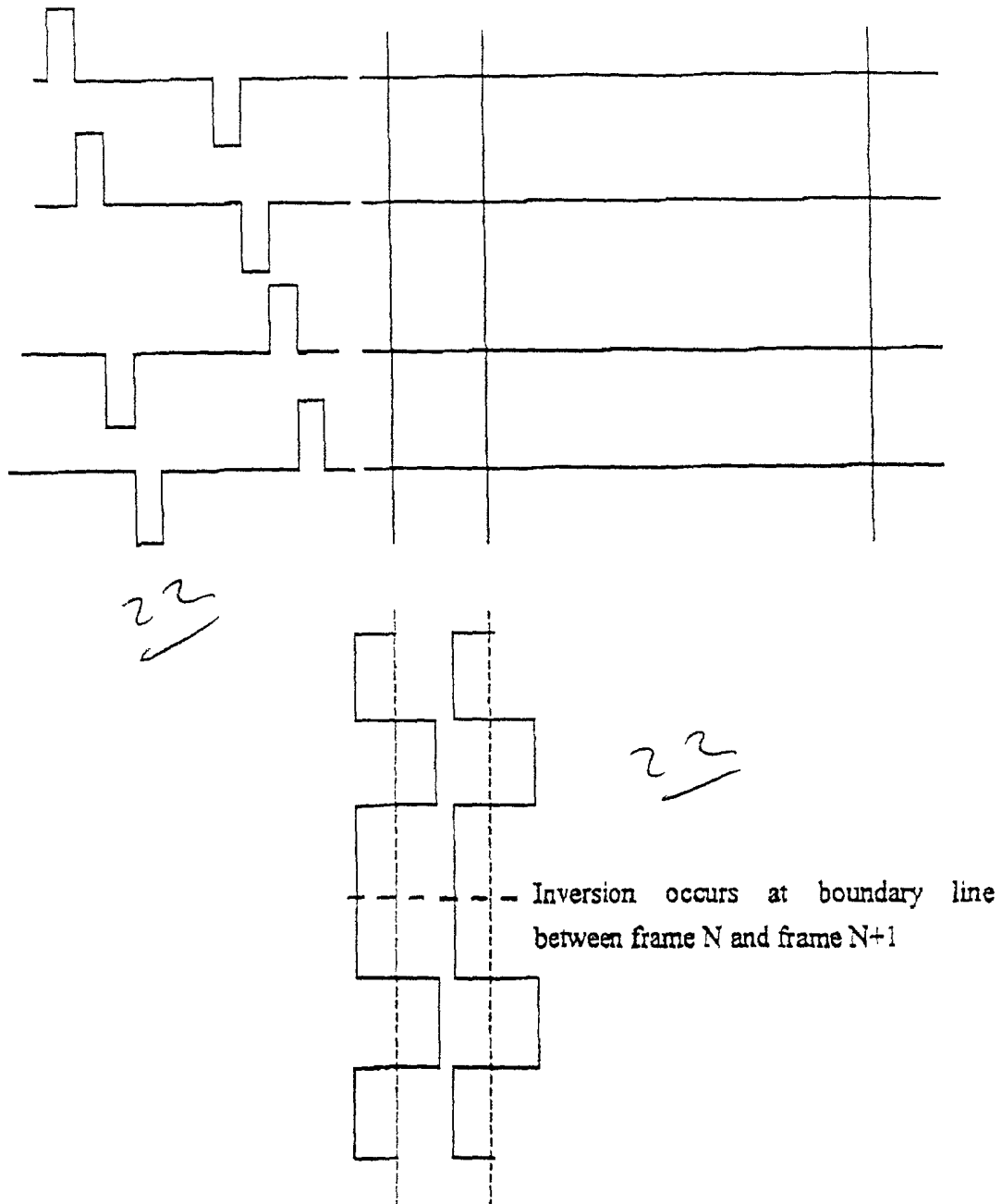
Fig. 15 Signal waveform incorporating 2-row inversion scheme for passively driven liquid crystal display
