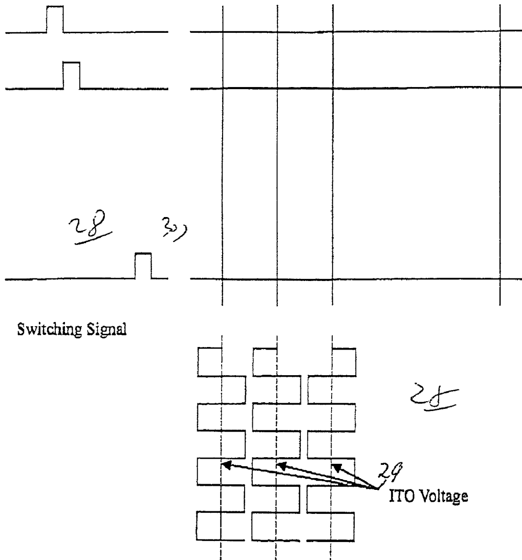
Fig. 21 Signal waveform incorporating 2x2-pixel inversion scheme for actively driven liquid crystal display
