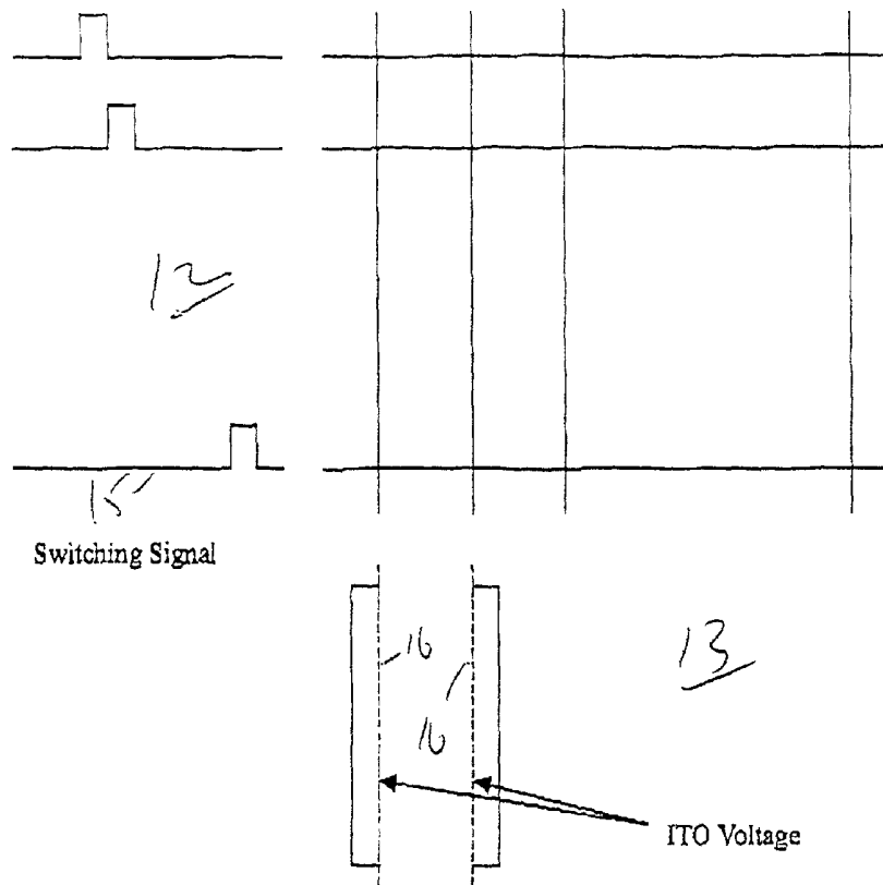
Fig. 8 Signal waveform incorporating column inversion scheme for actively driven liquid crystal display
