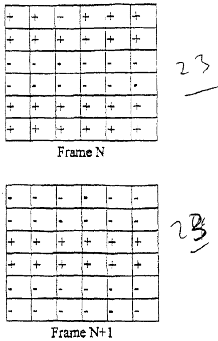
Fig. 16 Polarities of resulting fields applied to pixels for two consecutive frames adopting 2-row inversion scheme
