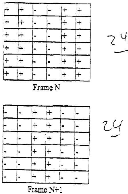
Fig. 17 Polarities of resulting fields applied to pixels for two consecutive frames adopting 2-column inversion scheme
