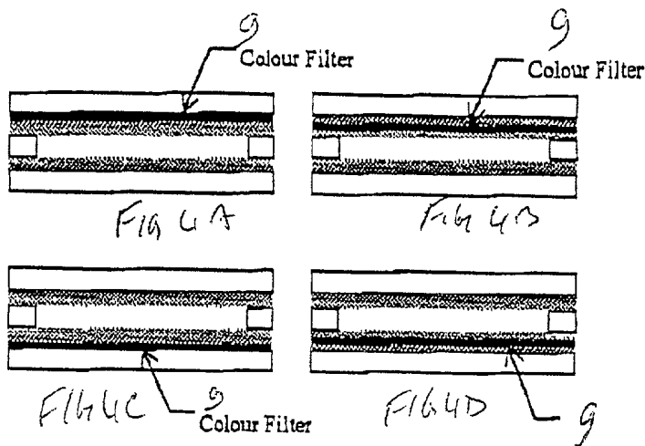
Fig. 4 Color filter material applied on/under the ITO layer
