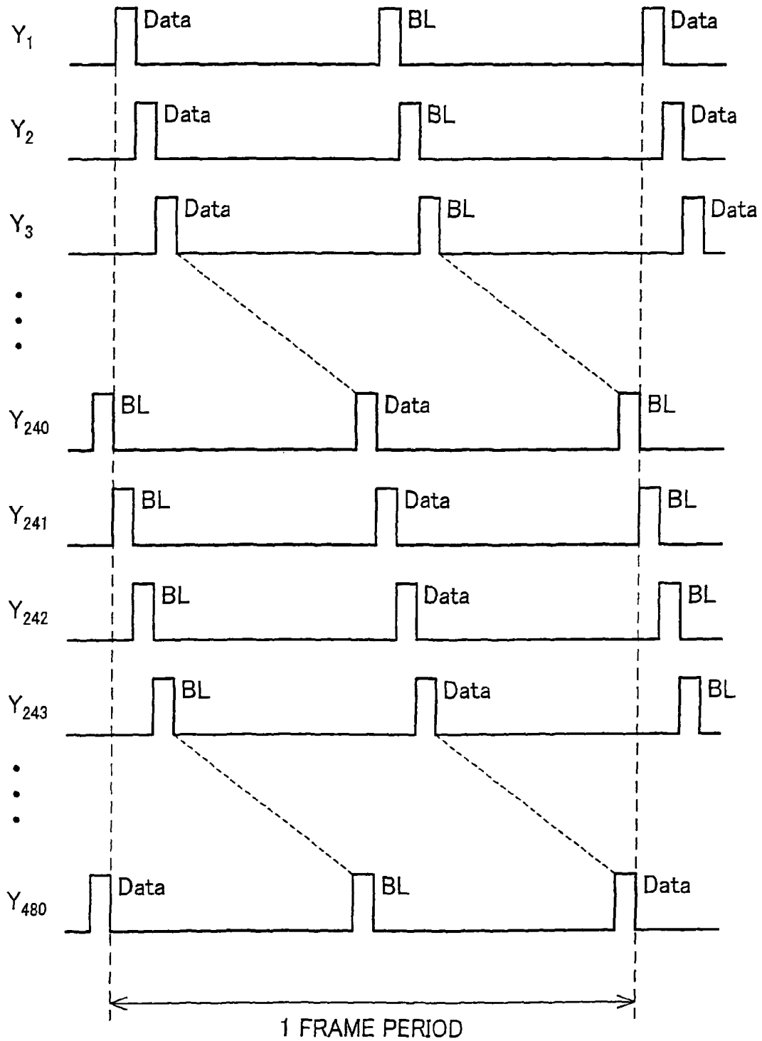
FIG. 11 (Conventional Art)
