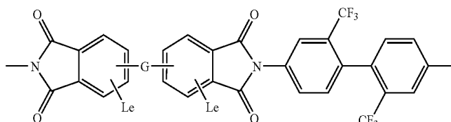
[Chemical Formula 2]
