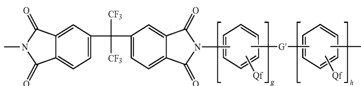
[Chemical Formula 2]
