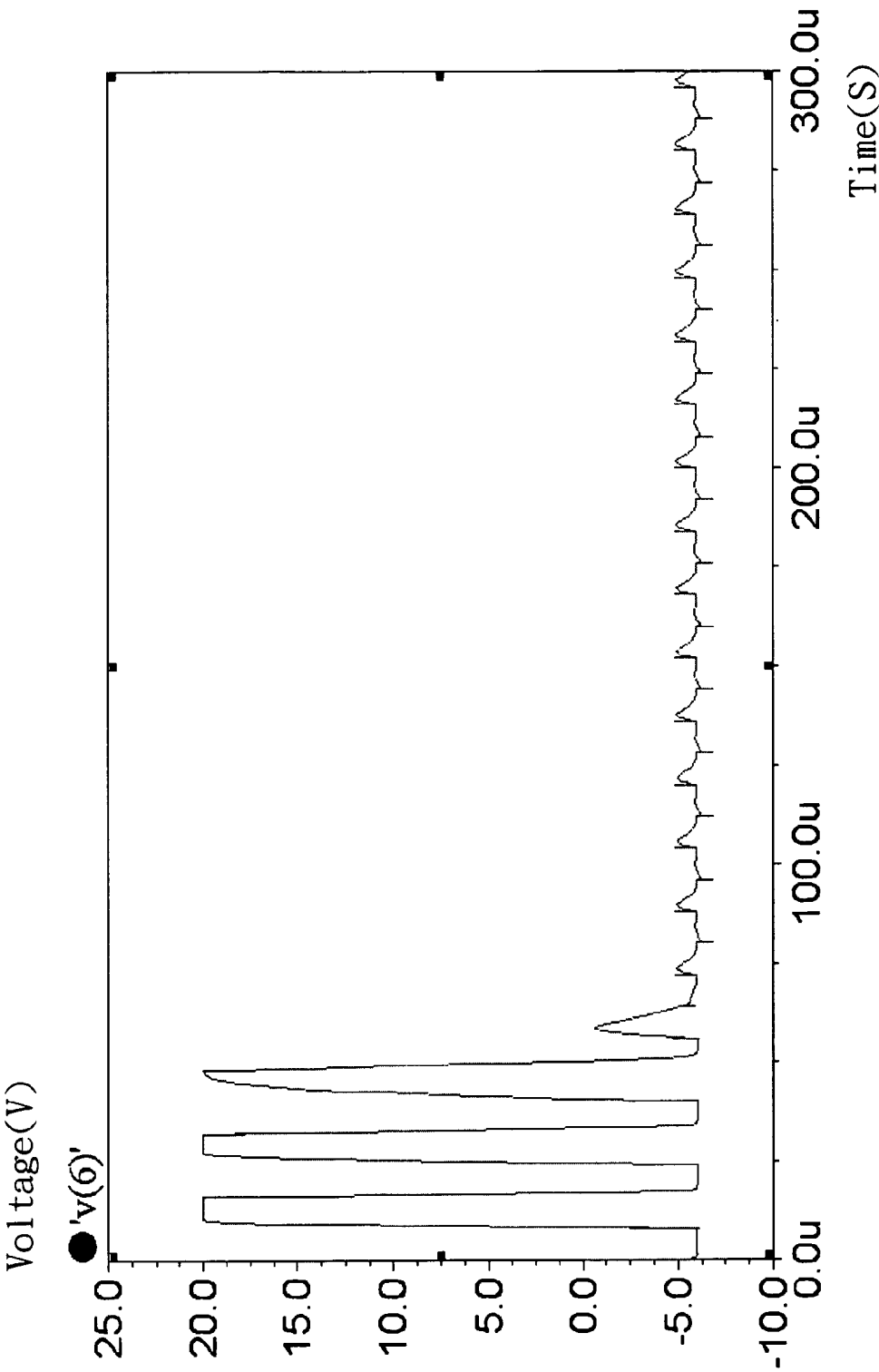
FIG. 4(RELATED ART)
