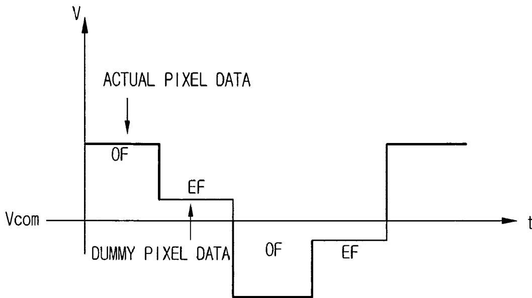
Fig.5 Related Art
