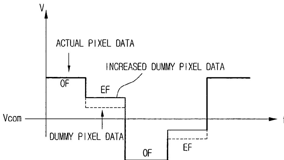
Fig.6 Related Art
