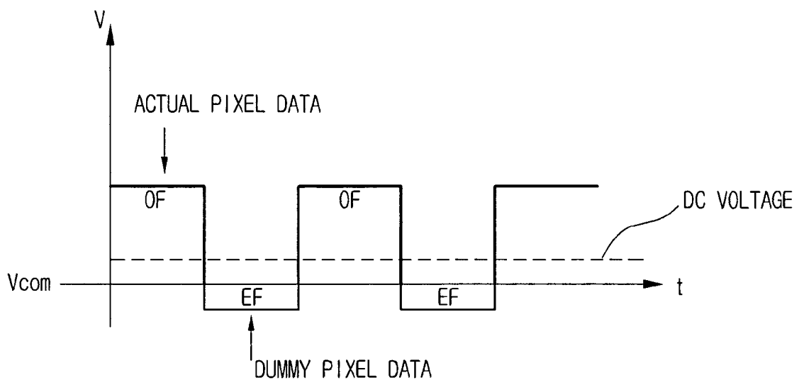
Fig.3 Related Art
