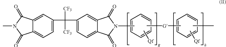
[Chemical Formula 2]
