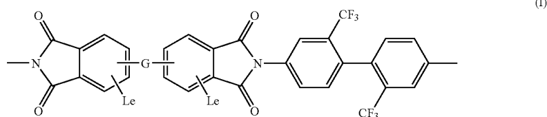
[Chemical Formula 2]
