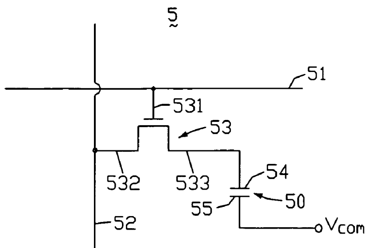
FIG. 5 (RELATED ART)
