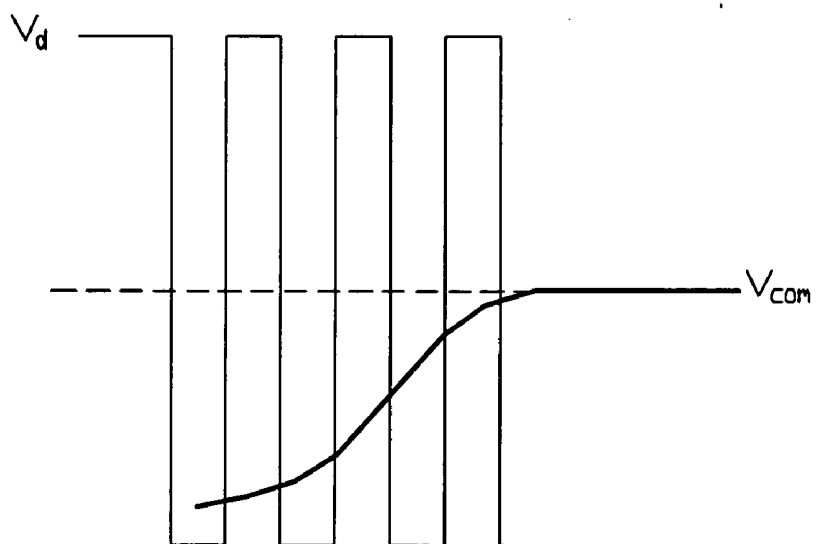
FIG. 6 (RELATED ART)
