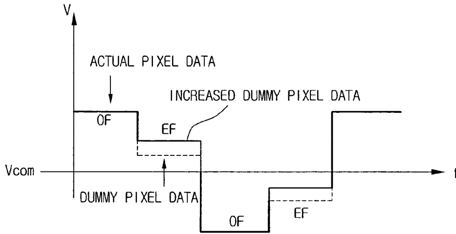
Fig.6 Related Art
