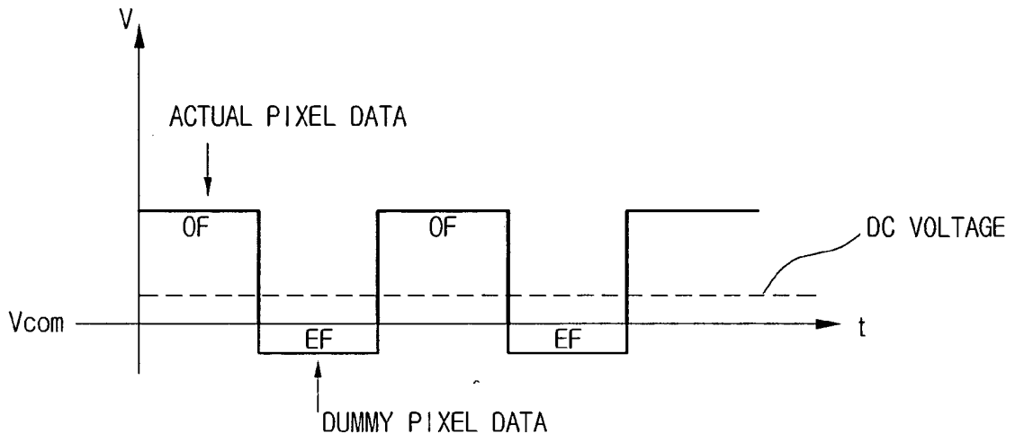
Fig.3 Related Art
