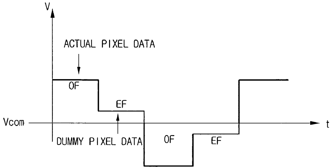
Fig.5 Related Art
