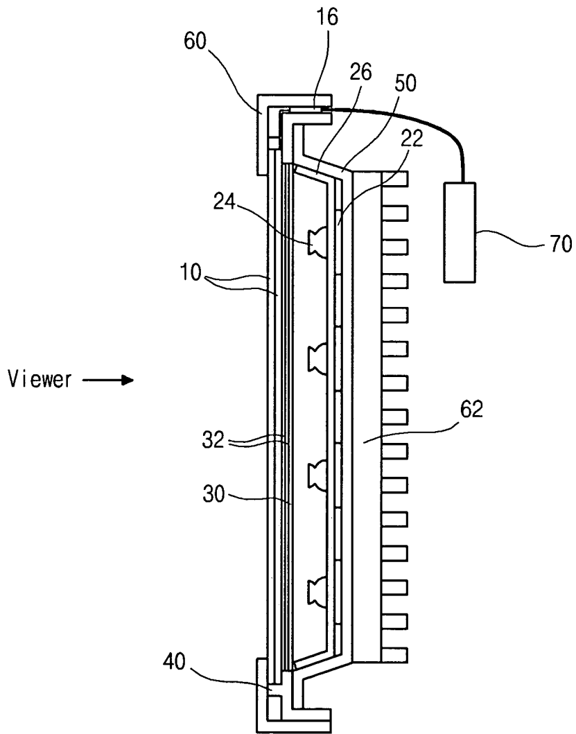
FIG. 2 RELATED ART
