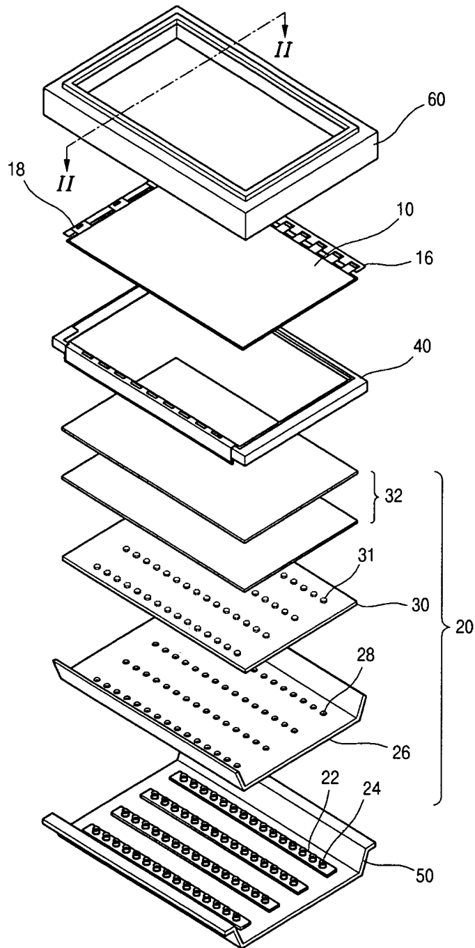
FIG. 1 RELATED ART
