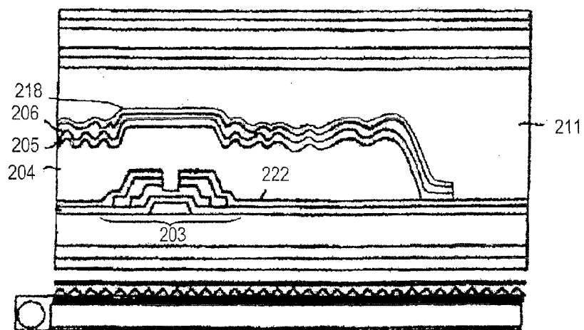
FIG. 12 (Prior Art)
