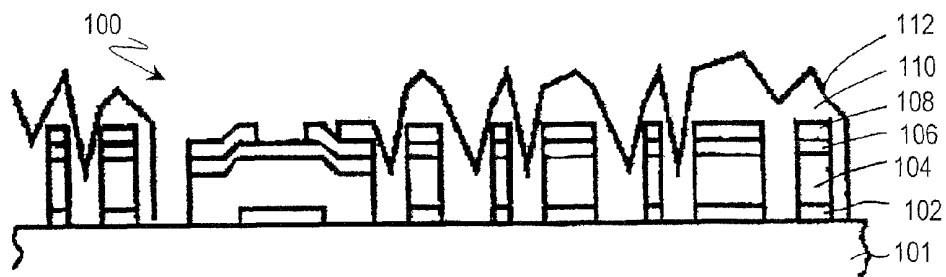
FIG. 11 (Prior Art)
