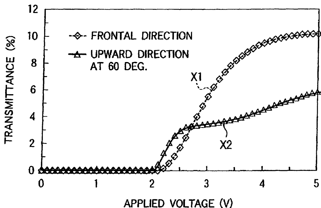
FIG.18 PRIOR ART
