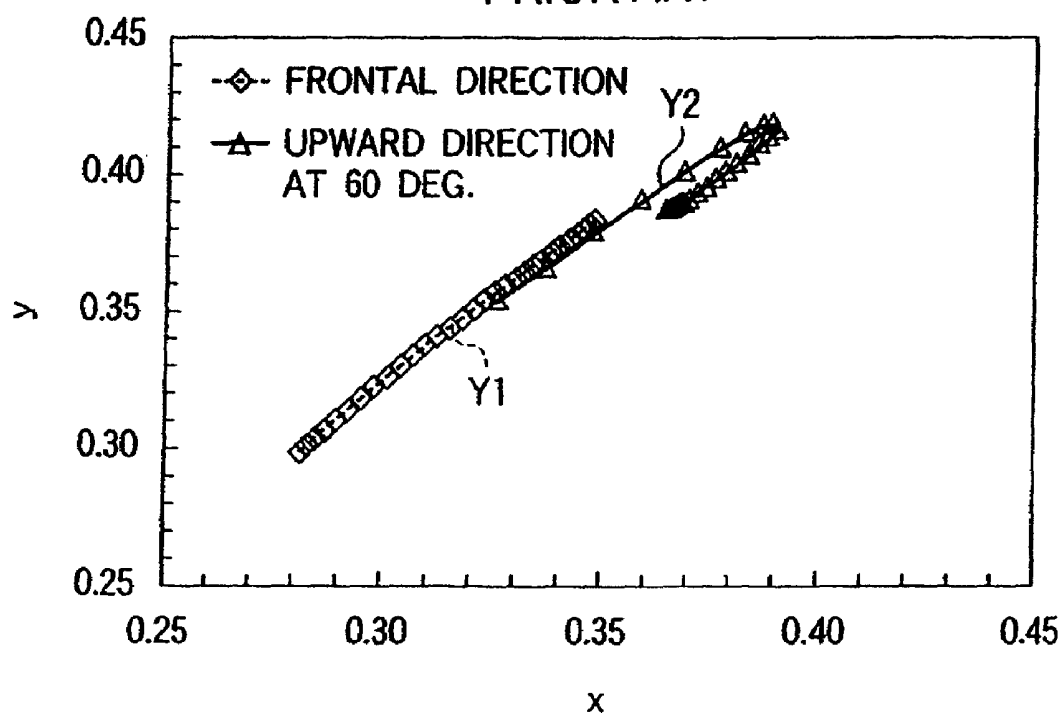
FIG.19 PRIOR ART
