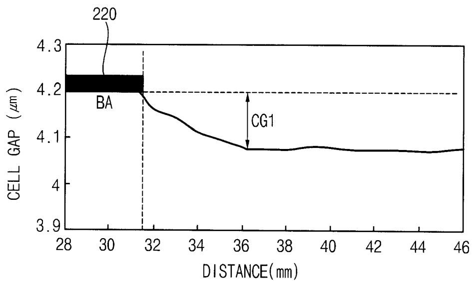
FIG. 9 (PRIOR ART)
