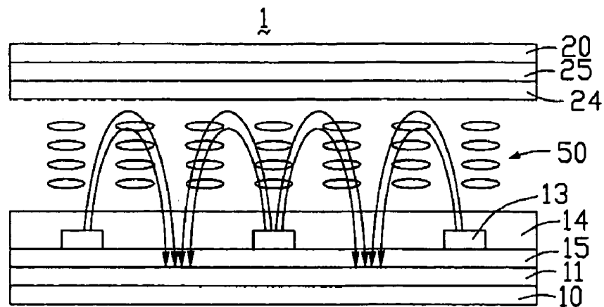
FIG. 4 (PRIOR ART)
