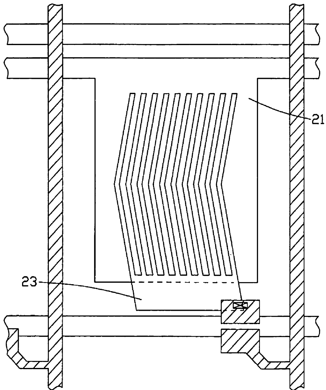
FIG. 6 (PRIOR ART)
