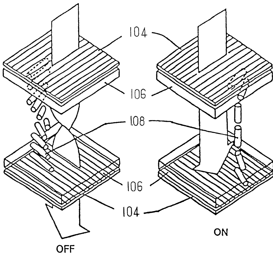
FIG. 3 (PRIOR ART)
