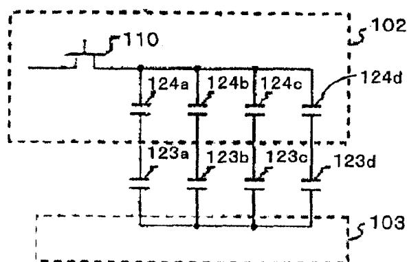
PRIOR ART FIG.36C
