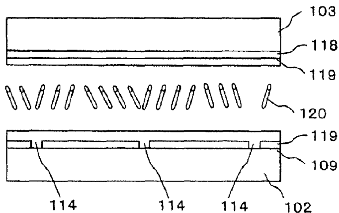
PRIOR ART FIG.34C
