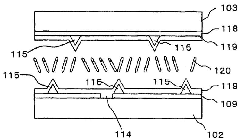
PRIOR ART FIG.34C
