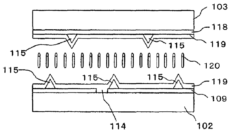
PRIOR ART FIG.34A
