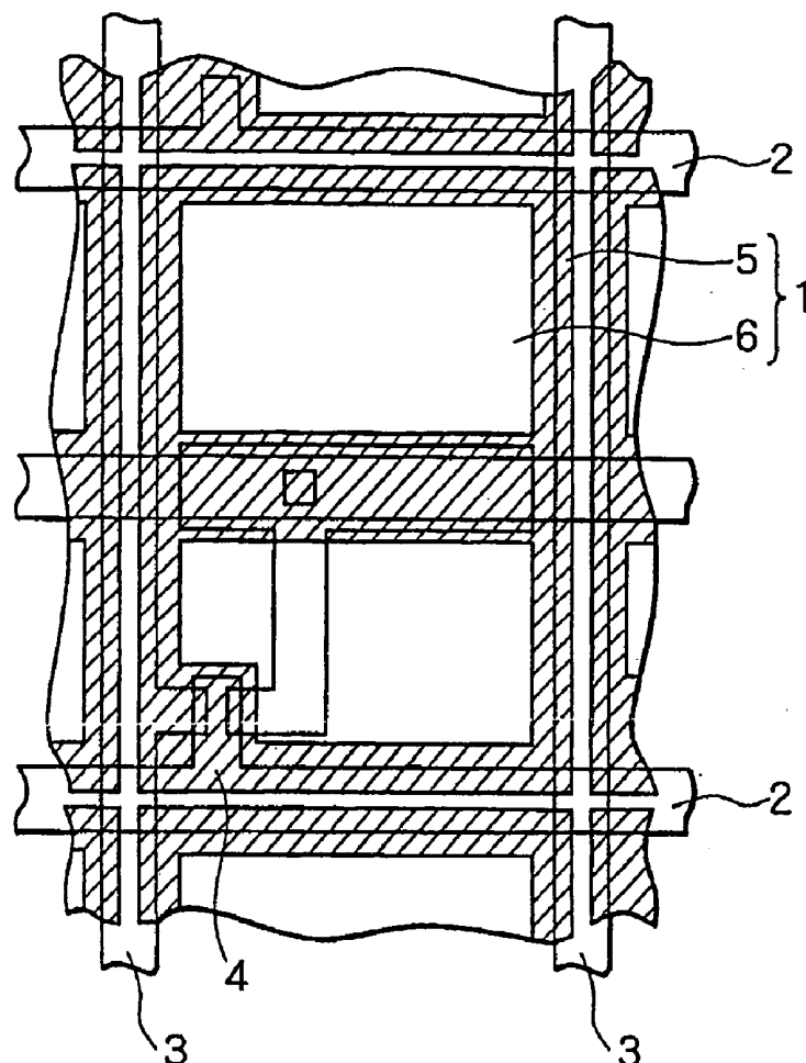
FIG. 1 (PRIOR ART)
