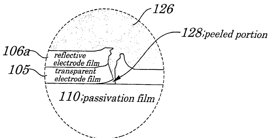
FIG. 31C(PRIOR ART)
