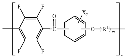
[Chemical formula 7]
