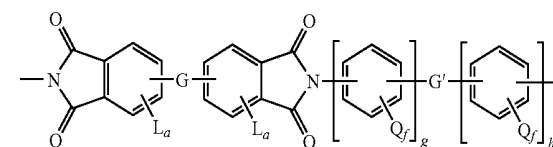
[Chemical formula 4]
