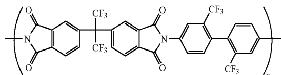
[Chemical formula 6]
