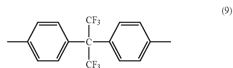
[Chemical formula 9]
