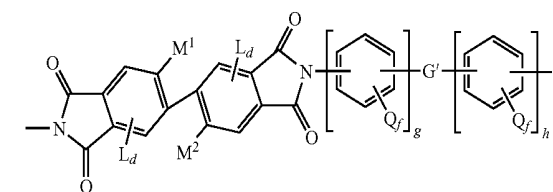
[Chemical formula 5]
