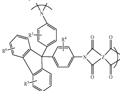
[Chemical formula 1]
