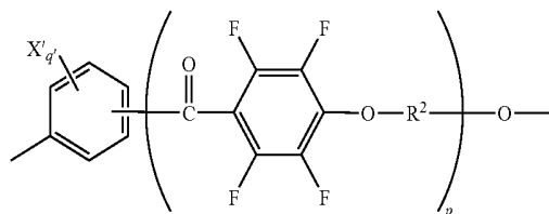
[Chemical formula 8]
